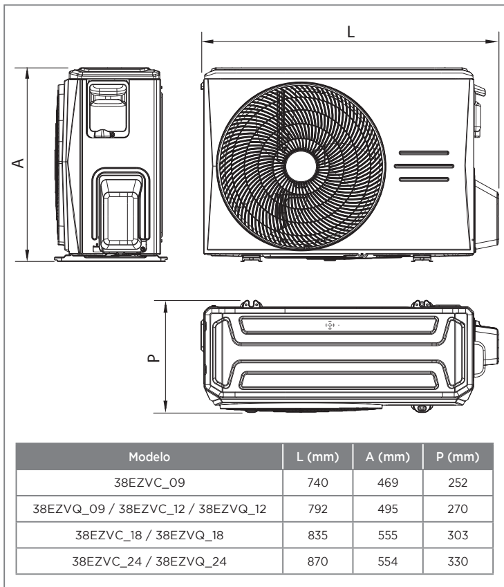
FIG. 4 - DIMENSIONAL
