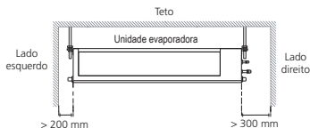
FIG. 35 - DIMENSIONAL
