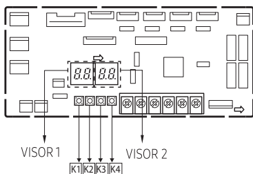
PCB PRINCIPAL - SAÍDA
